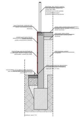
railings _ mounting detail
